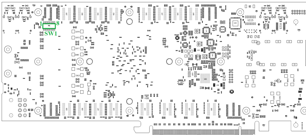
Figure 9 : Switches
