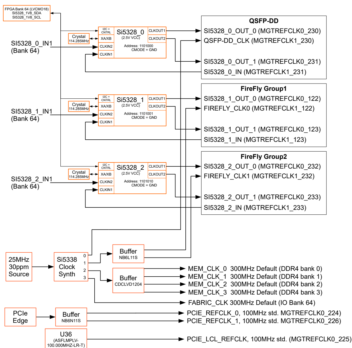
Figure 11 : Clock Topology
