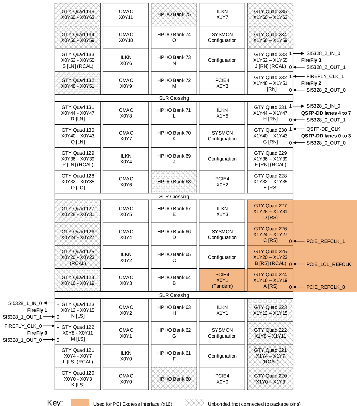
Figure 13 : VU13P FPGA Clock Location
