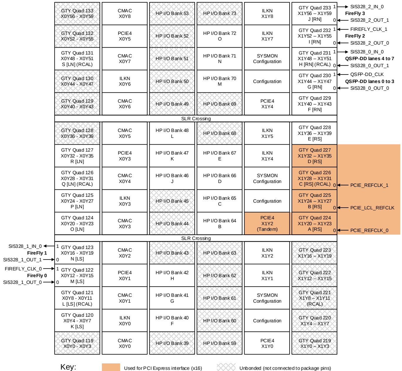
Figure 12 : VU9P FPGA Clock Location
