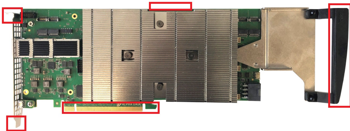
Figure 5 : Retention Points
