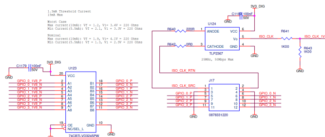
Figure 18 : GPIO Connector Schematic
