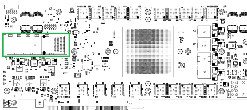
Figure 15 : QSFP-DD Location
