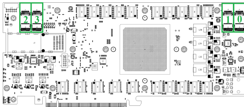
Figure 16 : FireFly Locations
