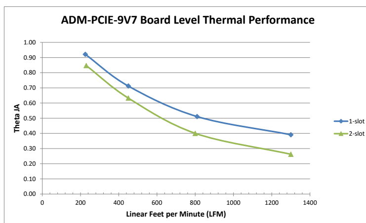
Figure 6 : Thermal Performance
